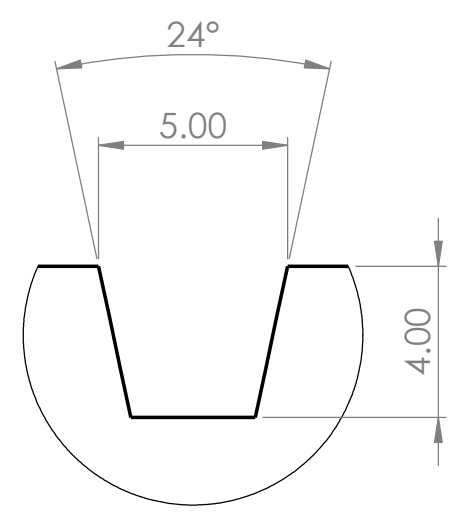
DETAIL B SCALE 5 : 1
